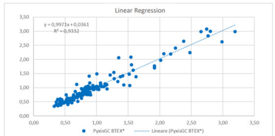
Graph 6 - Calculation of linear regression between instrumental measurements (Benzene concentrations expressed in ug/m 3 ) Week 2
