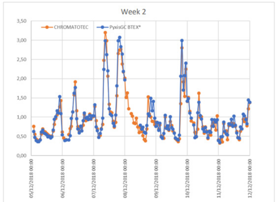
Graph 5 - Hourly average Benzene trend (concentrations expressed in ug / m 3 ) Week 2
