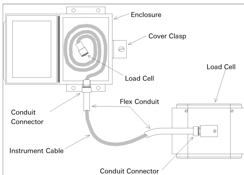
FIGURE 5: Typical Load Cell System
